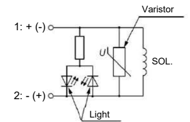
Figure 12. DIN terminal with light and surge voltage suppressor
