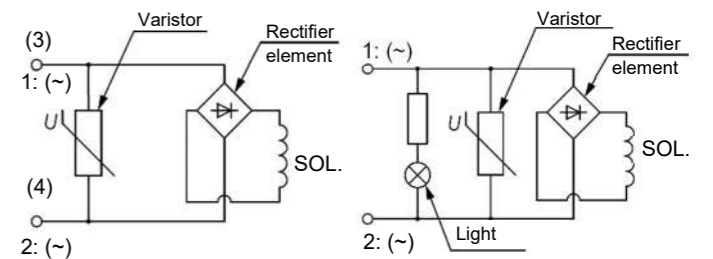
Figure 13. Grommet / DIN terminal / Conduit with surge voltage suppressor / M12 connector (3,4) Figure 14. DIN terminal with light and surge voltage suppressor
