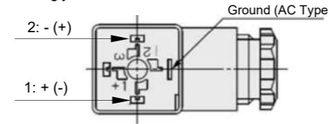
Figure 9. DIN connector pins
