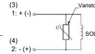
Figure 11. Grommet / DIN terminal / Conduit with surge voltage suppressor / M12 connector (3,4)
